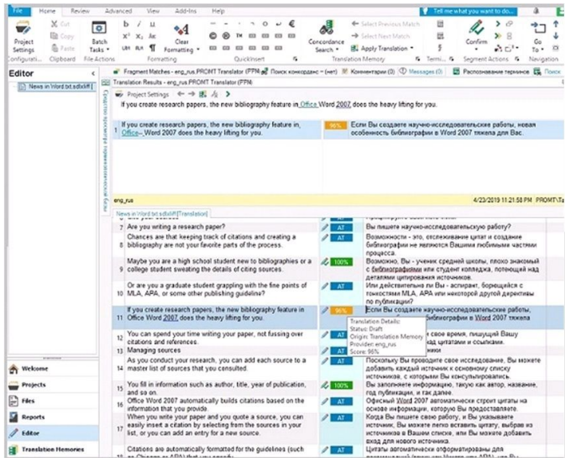
Fig. 4.11. Translation Results
