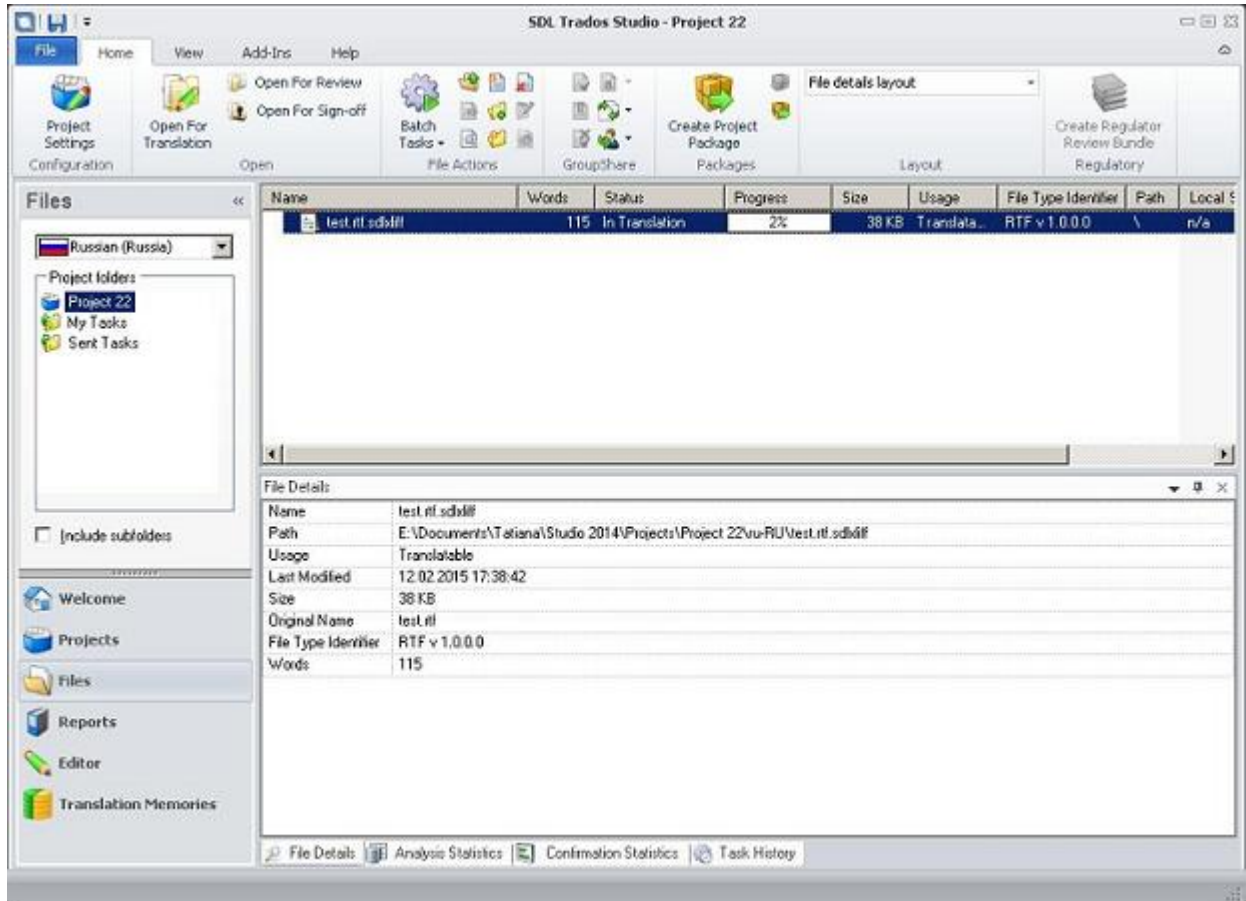
Fig. 3.4. File Details
