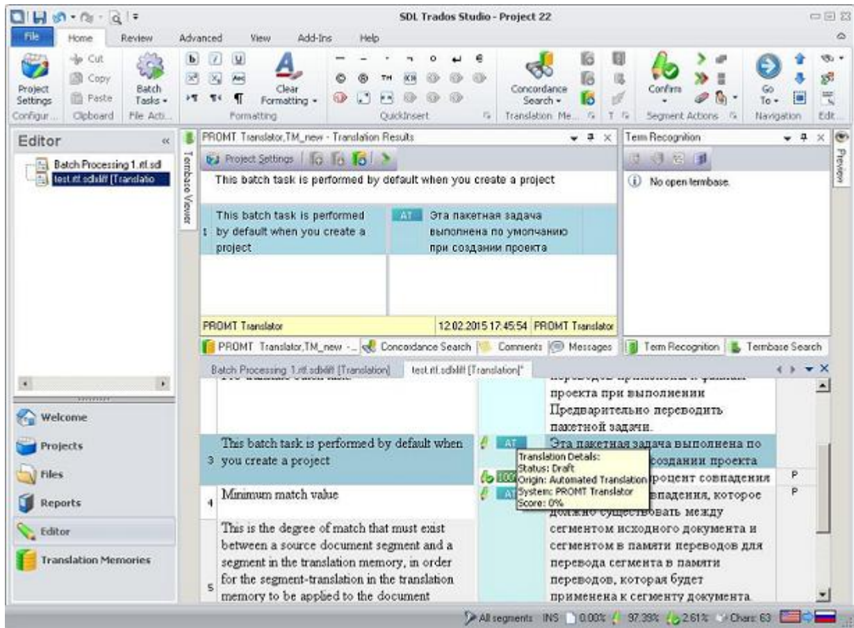
Fig. 3.5. Translation Results
